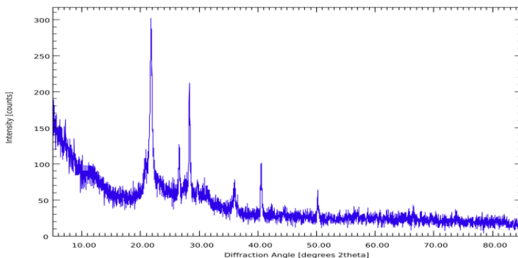
Figure 5. X-ray diffraction peak distribution for rice straw ash
