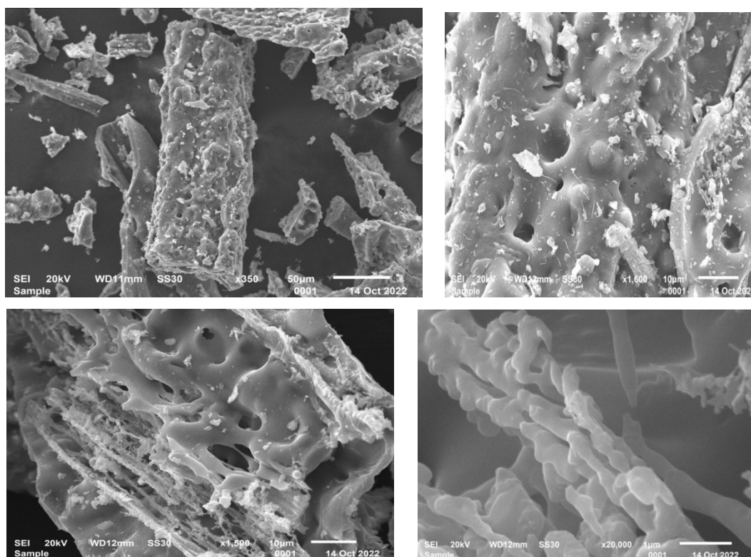
Figure 9. Scanning electron micrographs of RSA
