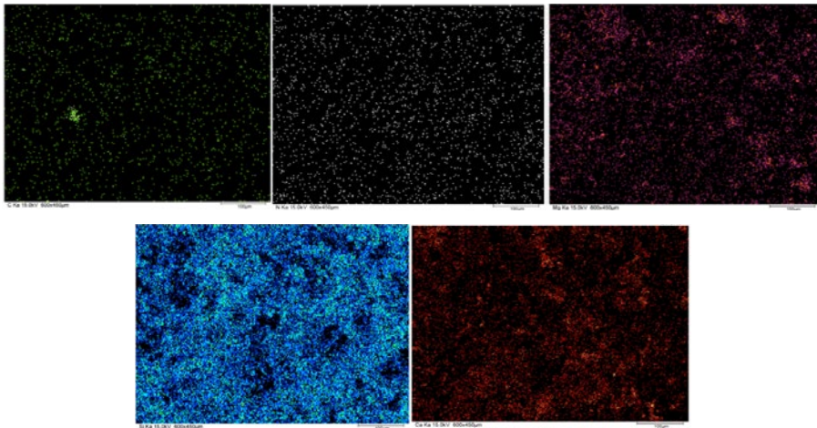
Figure 7. Wavelength-dispersive spectrometry (WDS) intensity map (600x450µm) of C, N, Mg, Si and Ca
