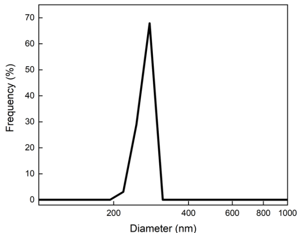
Figure 11. Dynamic Light Scattering analysis of RSA
