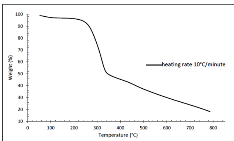
Figure 4. Thermogravimetric analysis curve showing weight loss (in %) of Rice Straw over time at a constant heating rate from 50°C to 800°C at 10°C per min
